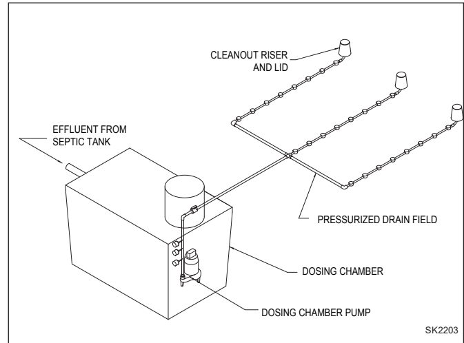
Typical Pressure Distribution System
